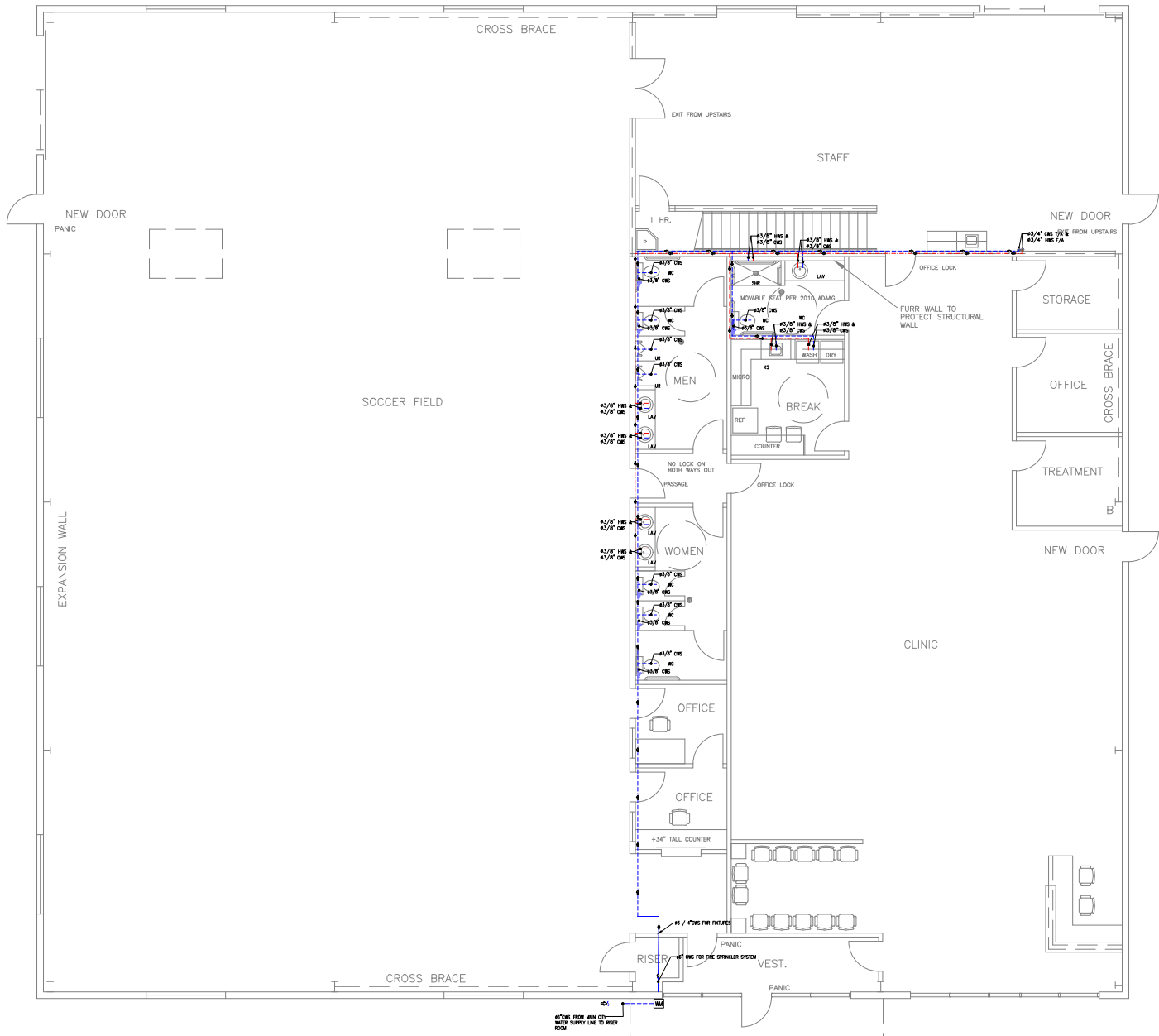
PL 03 FIRST FLOOR WATER SUPPLY PLAN SCALE 1/16"=1'-0"
