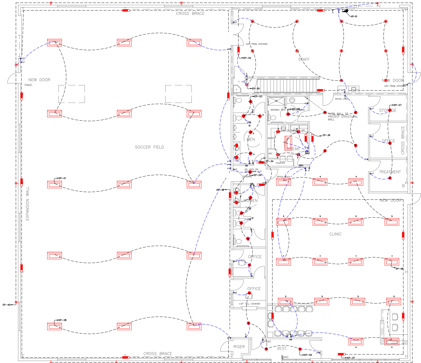
EL 02 SCALE 1/16"=1'-0" FIRST FLOOR LIGHTING PLAN
