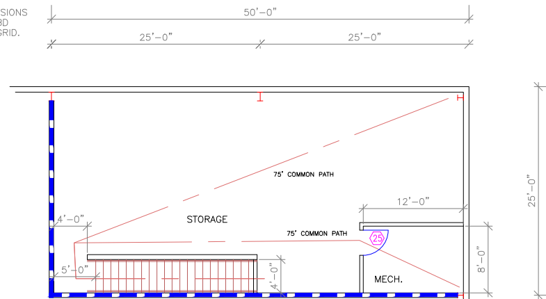
AR 02 SCALE 1/16"=1'-0" SECOND FLOOR PLAN
