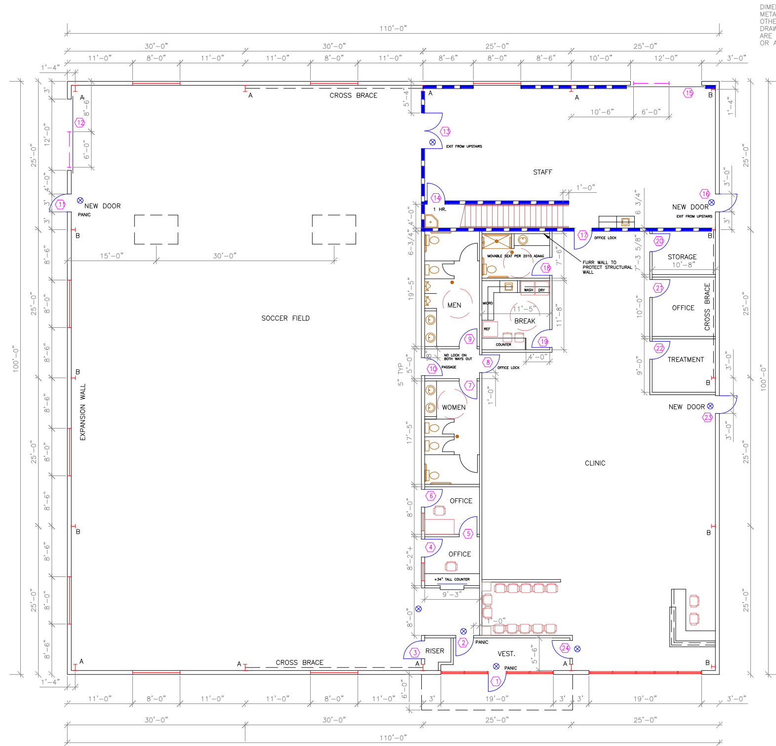
AR 02 SCALE 1/16"=1'-0" FIRST FLOOR PLAN
