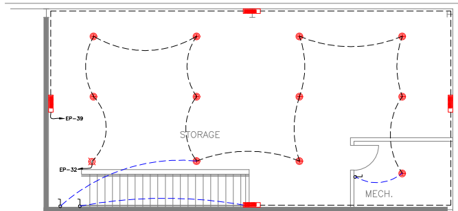
EL 02 SCALE 1/16"=1'-0" SECOND FLOOR LIGHTING PLAN
